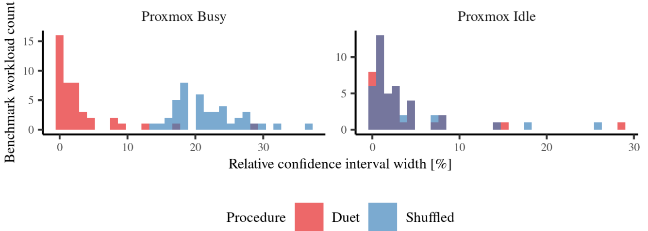
Figure 5: Impact of resource sharing on random shuffling in private cloud, idle vs busy with competing workload, expressed as relative 99% confidence interval width, 10 runs, aggregated across all workloads.
